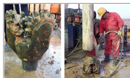
Figure 23 Condition of bit B after field test (see online version for colours)
